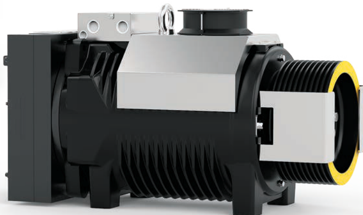
SG58F Gearless with fan kit
