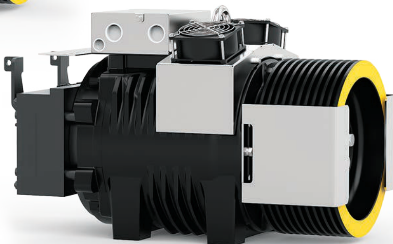
SG22F Gearless with fan kit
