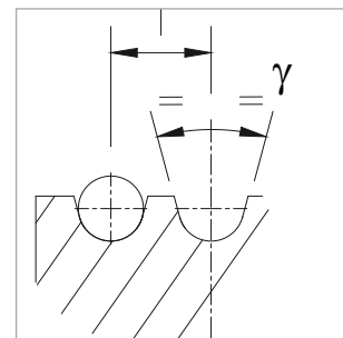
U grooves without undercut
