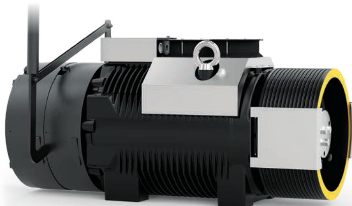
SG75F Gearless with fan kit
